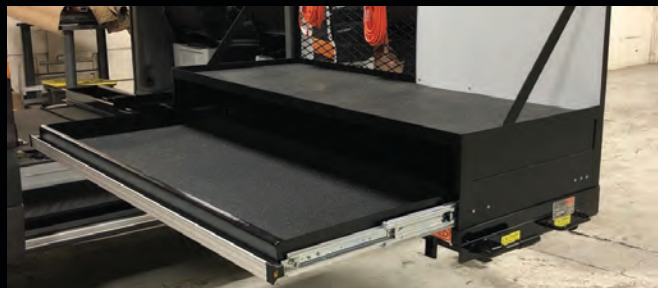
EXTENDOWALL IN VAN-SIDE DOOR MOUNT
